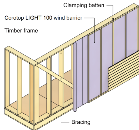
Fig. 1 Corotop LIGHT 100 used as wind barrier in a timber frame wall
