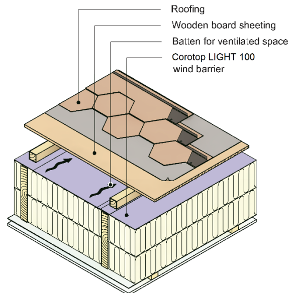
Fig. 2 Corotop LIGHT 100 used as wind barrier in an insulated and ventilated roof construction with a rain tight layer above.
